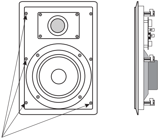
Mounting screws (6)
