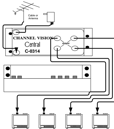
Standard Wiring Layout
